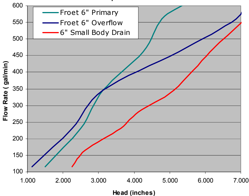
6" Froet Drain Flow Rate Comparison GPM verse Required Head in Inches
